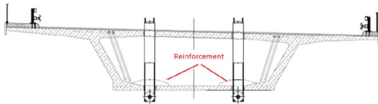
Figure 3. Pulling stick installation and segment reinforcement
